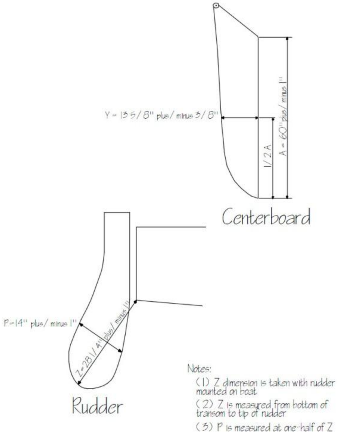
Figure 3. Rudder and Centerboard Certified Measurements
