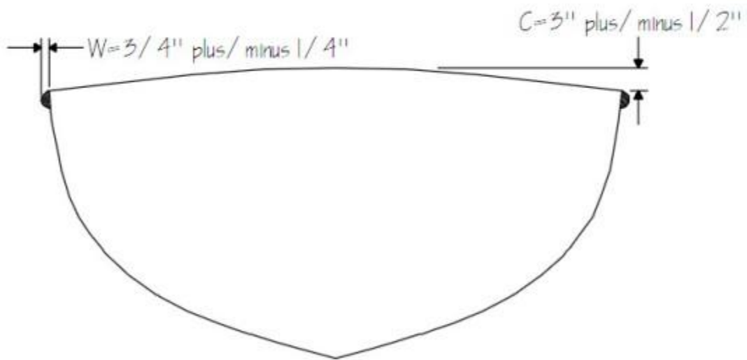
Section at Station 6
