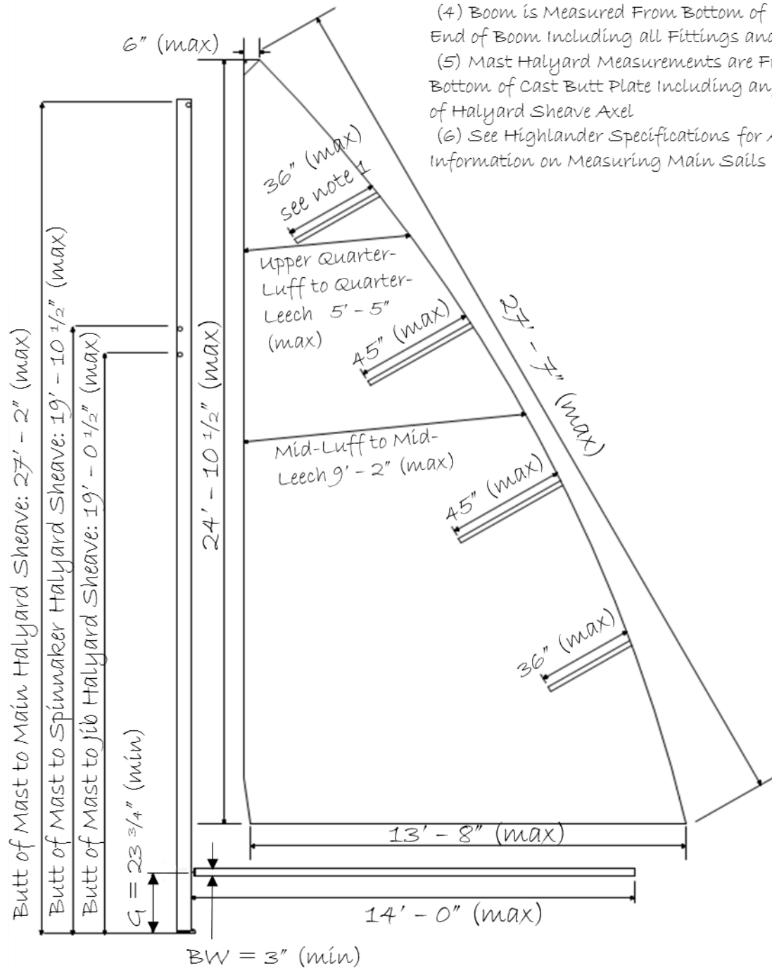
Figure 4 Mast, Mainsail and Boom Measurements
